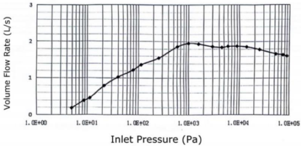
Inlet Pressure, Volume Flow Rate- Curve Table
