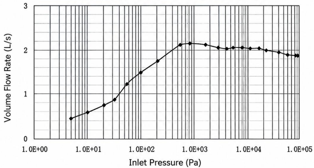
Inlet Pressure, Volume Flow Rate- Curve Table
